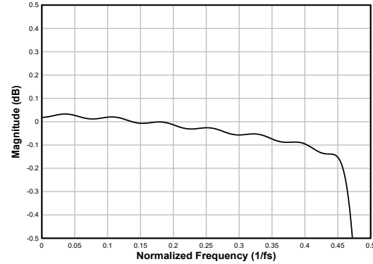
Figure 8-19. Linear Phase Interpolation Filter Pass-Band Ripple
