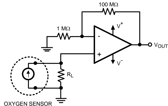
Figure 34. Precision Oxygen Sensor
