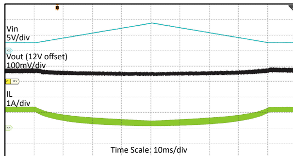
V_{IN} = 2.6V \text{ to } 9V V_{OUT} = 12V I_{OUT} = 200mA
