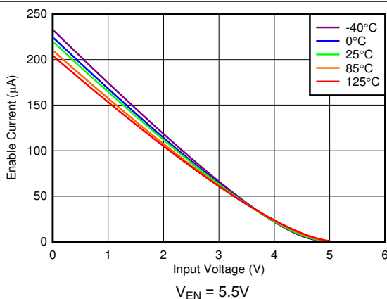
V_{EN} = 5.5\text{V} Figure 5-23. I_{EN} vs V_{IN}
