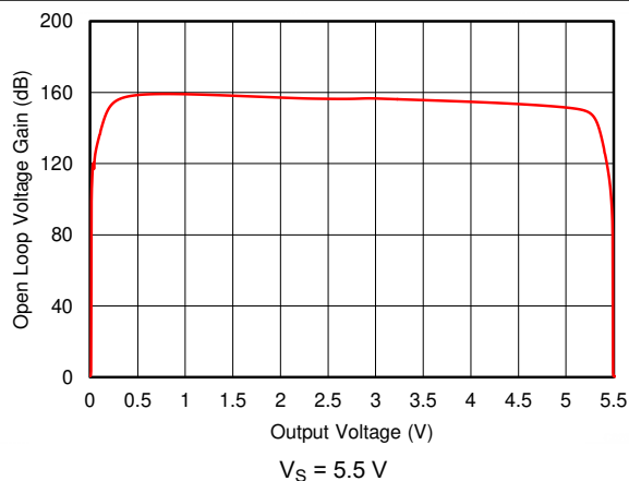
Figure 8-34. Open Loop Voltage Gain vs Output Voltage
