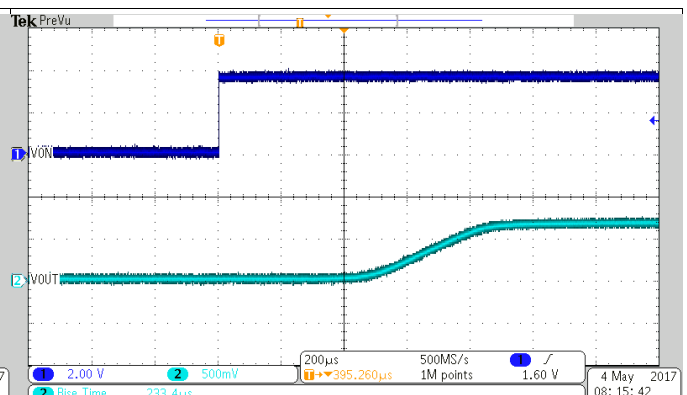
Figure 10. Turn-ON Response at 3.6 VIN
