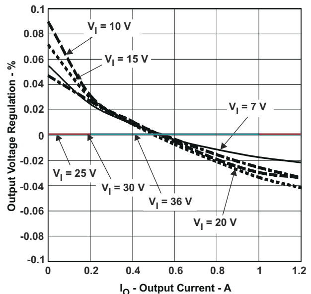
Figure 8-14. Output Voltage Regulation % vs. Output Current
