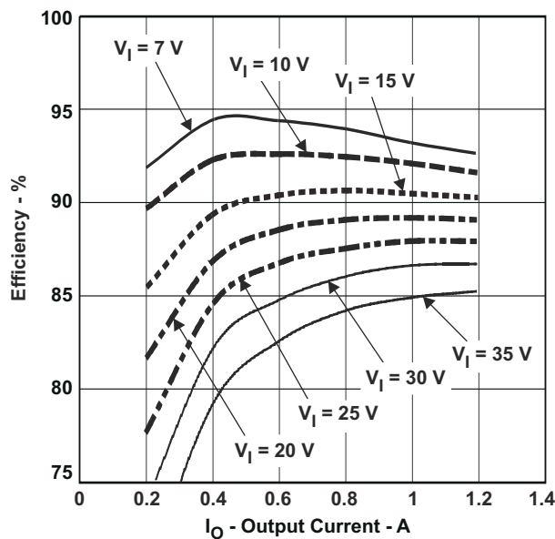
Figure 8-13. Efficiency vs. Output Current
