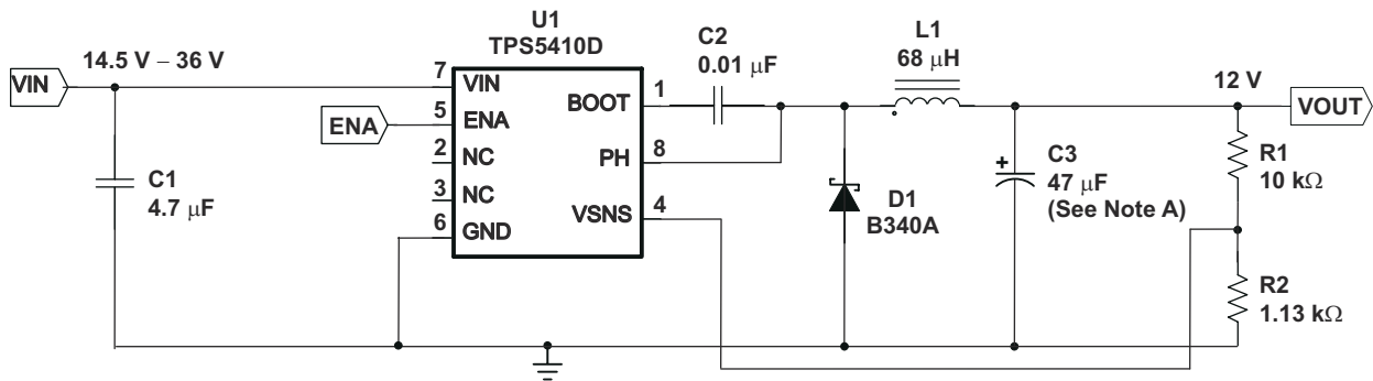
Figure 8-3. Application Circuit, 14.5-V — 36 V to 12-V
