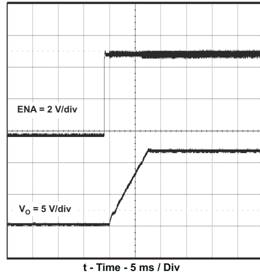
Figure 8-12. Startup Waveform, ENA and V_O
