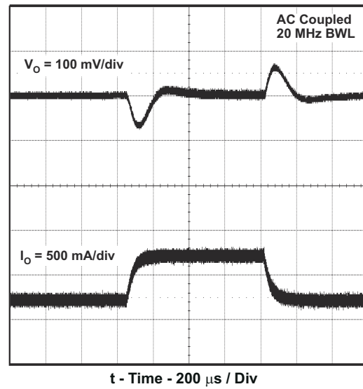
Figure 8-18. Transient Response, I_O Step 0.25 to 0.75 A
