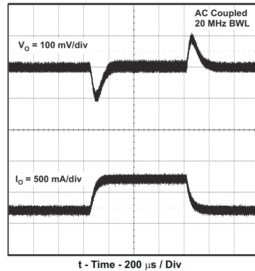
Figure 8-10. Transient Response, I_O Step 0.25 to 0.75 A
