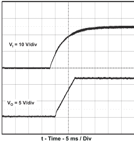
Figure 8-11. Startup Waveform, V_I and V_O
