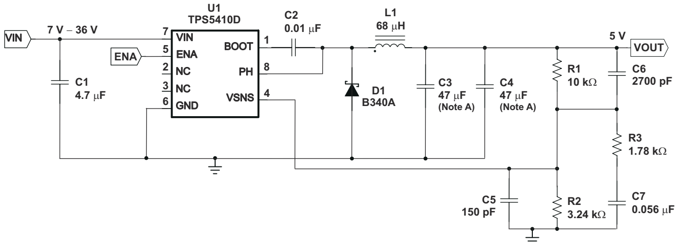
Figure 8-4. 7-V — 36-V Input to 5-V Output Application Circuit with Ceramic Capacitors
