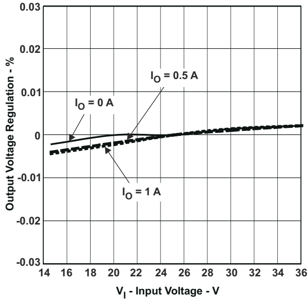
Figure 8-15. Output Voltage Regulation % vs. Input Voltage
