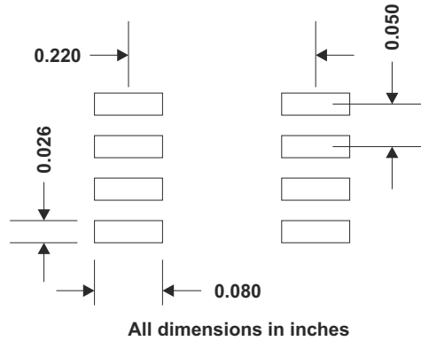
Figure 8-2. TPS5410 Land Pattern
