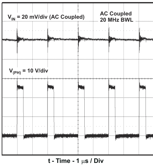
Figure 8-17. Output Voltage Ripple and PH Node, I_O = 1 A
