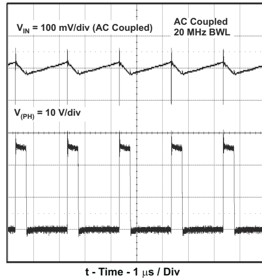
Figure 8-16. Input Voltage Ripple and PH Node, I_O = 1\text{ A}
