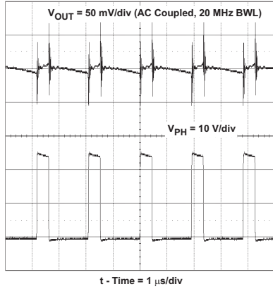
Figure 14. Output Voltage Ripple and PH Node
