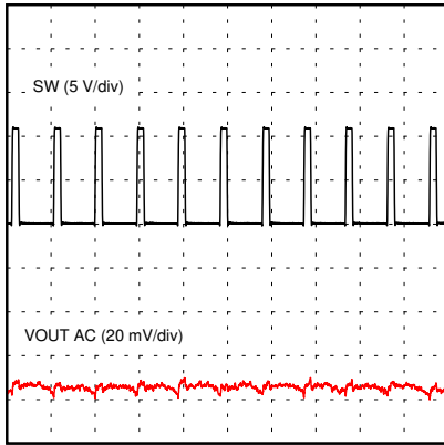
Figure 7-26. Output Voltage Ripple
