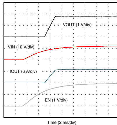
Figure 7-17. EN Start-Up – DCM
