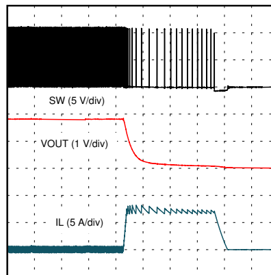
Figure 7-30. Short Circuit Response
