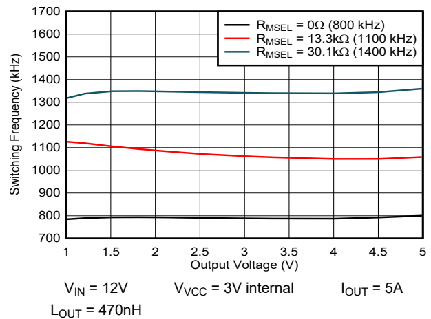
Figure 5-8. Switching Frequency versus Output Voltage
