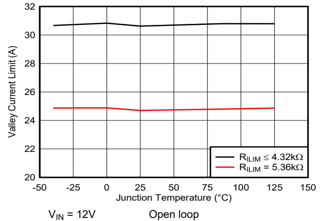
Figure 5-20. Valley Current Limit versus Junction Temperature (Low R_{ILIM} )
