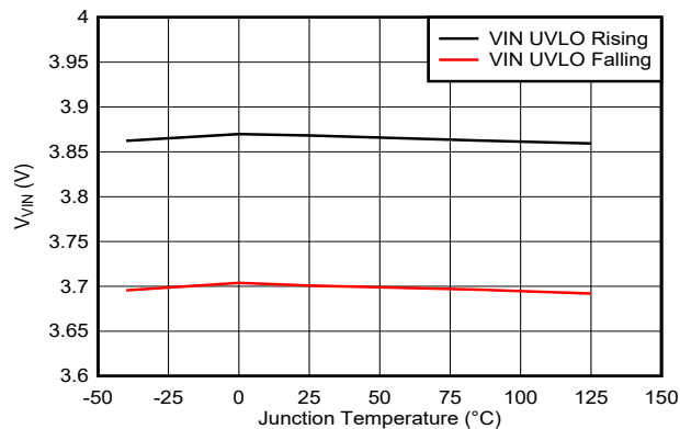
Figure 5-23. VIN Pin Undervoltage Lockout versus Junction Temperature
