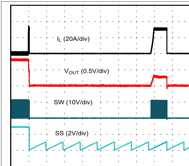
Figure 6-1. Entering Hiccup
