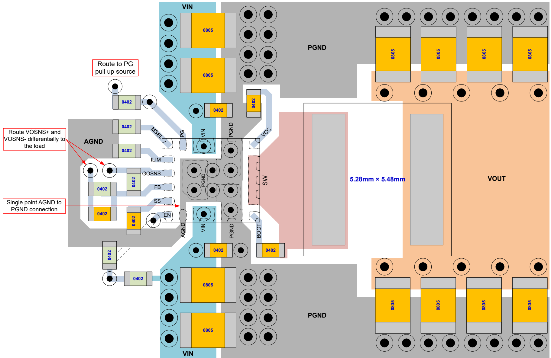
Figure 7-12. Layout Recommendation
