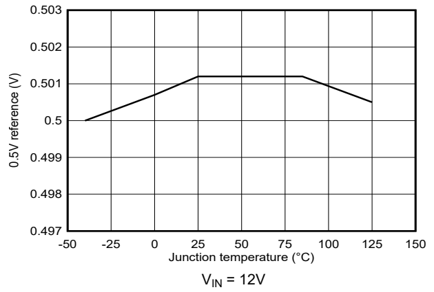
Figure 5-16. 0.5V Reference Voltage versus Junction Temperature
