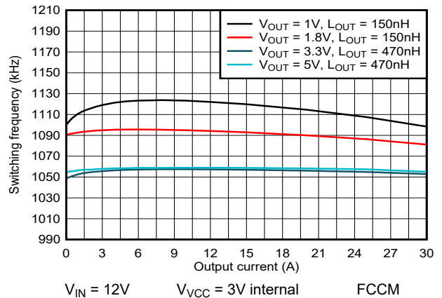
Figure 5-14. 1100kHz Switching Frequency versus Output Current
