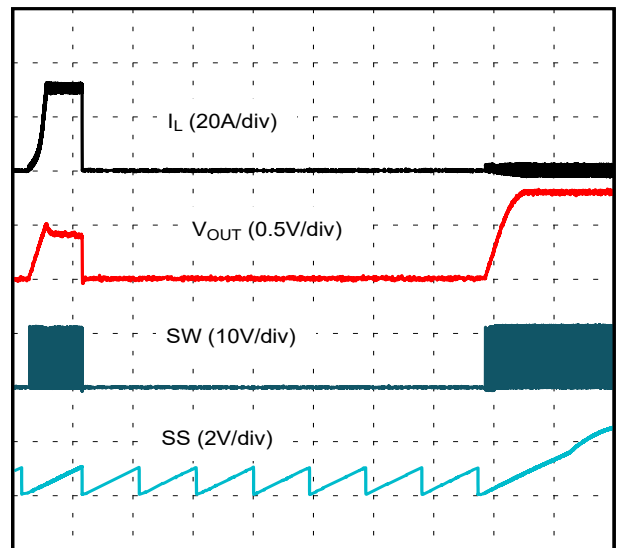
Figure 6-2. Exiting Hiccup
