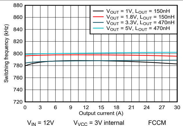
Figure 5-12. 800kHz FCCM Switching Frequency versus Output Current
