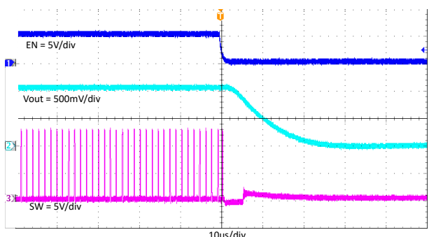
Figure 7-15. TPS563206 Enable off With 3A Loading
