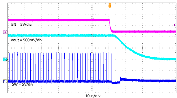
Figure 7-13. TPS563203 Enable off With 3A Loading
