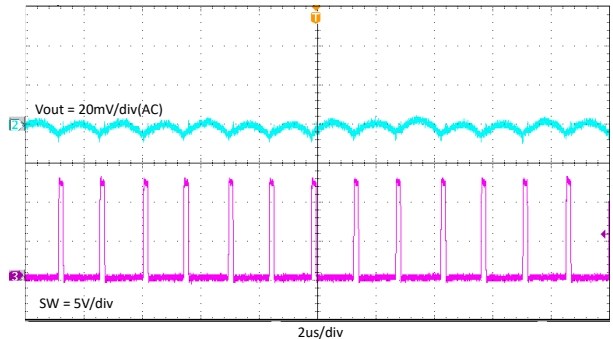
Figure 7-11. TPS563206 Output Voltage Ripple With 3A Loading
