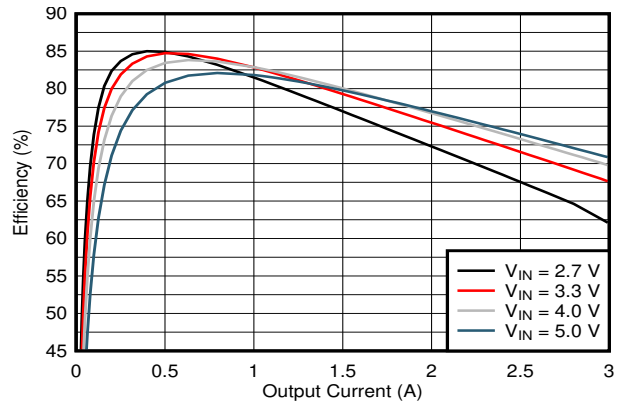
V_{OUT} = 0.6\text{ V} PWM T_A = 25^\circ\text{C} Figure 9-9. Efficiency Versus Output Current
