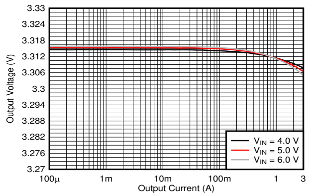
V_{OUT} = 3.3\text{ V} PWM T_A = 25^\circ\text{C} Figure 9-11. Output Voltage Versus Output Current
