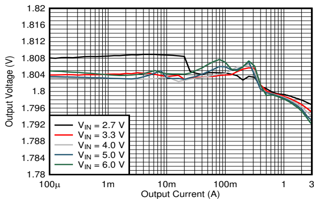
V_{OUT} = 1.8\text{ V} PFM T_A = 25^\circ\text{C} Figure 9-12. Output Voltage Versus Output Current
