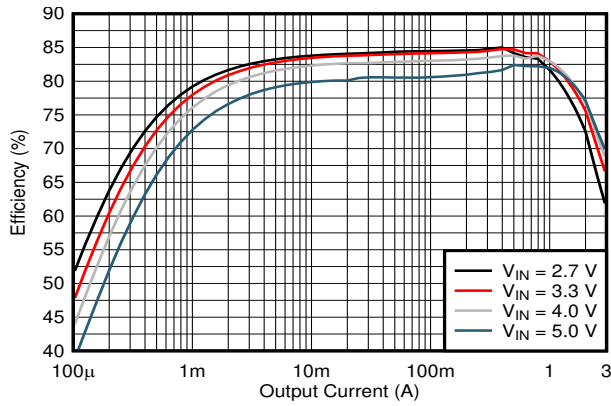
V_{OUT} = 0.6\text{ V} PFM T_A = 25^\circ\text{C} Figure 9-8. Efficiency Versus Output Current
