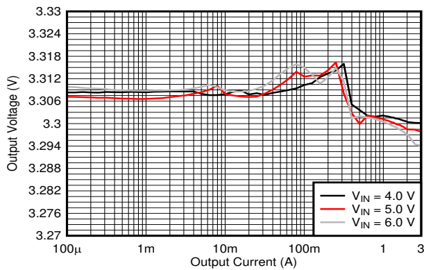
V_{OUT} = 3.3\text{ V} PFM T_A = 25^\circ\text{C} Figure 9-10. Output Voltage Versus Output Current
