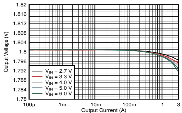
V_{OUT} = 1.8\text{ V} PWM T_A = 25^\circ\text{C} Figure 9-13. Output Voltage Versus Output Current
