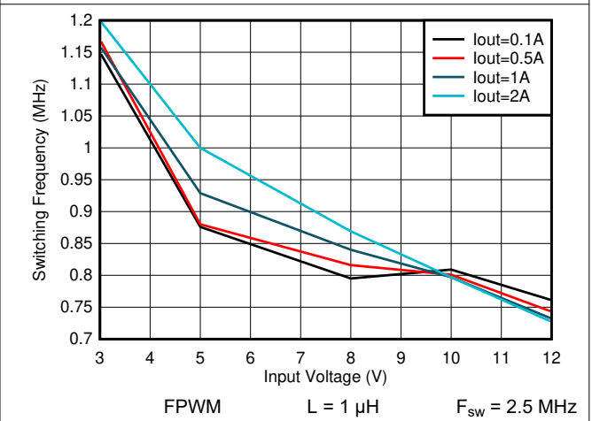
Figure 8-77. Switching Frequency vs Input Voltage V OUT = 0.4 V
