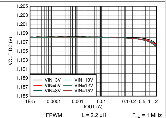
Figure 8-79. Output Voltage vs Output Current V OUT = 1.2 V
