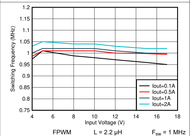
Figure 8-28. Switching Frequency vs Input Voltage V_{OUT} = 3.3 V
