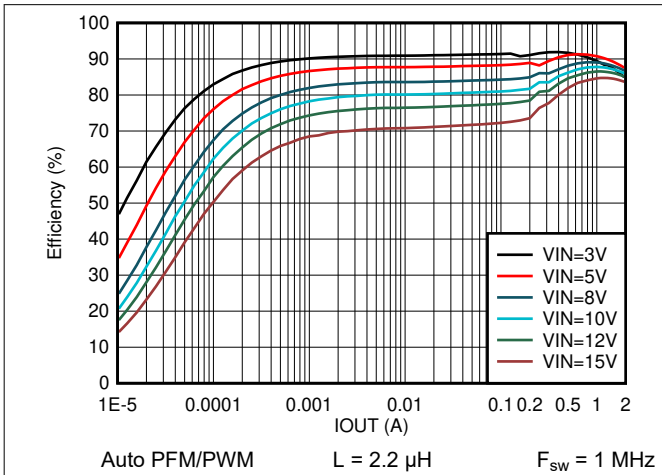
Figure 8-19. Efficiency vs Output Current V_{OUT} = 1.2 V
