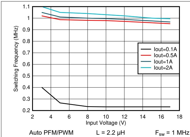
Figure 8-31. Switching Frequency vs Input Voltage V_{\text{OUT}} = 1.8 \text{ V}
