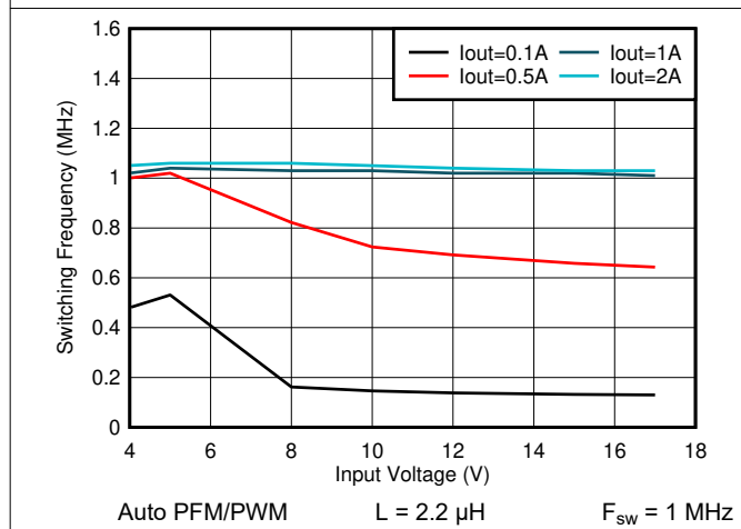
Figure 8-27. Switching Frequency vs Input Voltage V_{OUT} = 3.3 V
