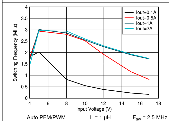
Figure 8-29. Switching Frequency vs Input Voltage V_{OUT} = 3.3 V
