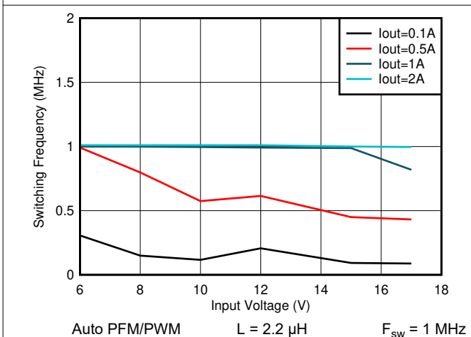
Figure 8-23. Switching Frequency vs Input Voltage V_{OUT} = 5 V
