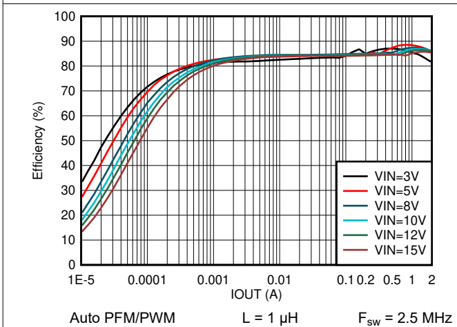
Figure 8-21. Efficiency vs Output Current V_{OUT} = 1.2 V
