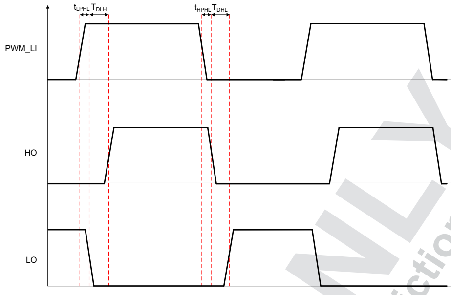
Figure 8-4. Timing Waveforms in PWM Mode Showing Dead Time
