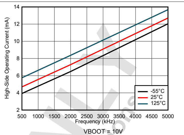
Figure 7-44. High-Side Operating Current vs Frequency (IIM)
