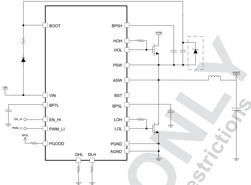
Figure 8-2. Direct VIN Bootstrap Charging Configuration
