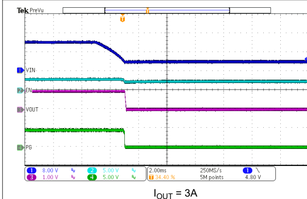
Figure 7-14. VIN Shutdown
