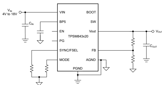
Simplified Schematic
