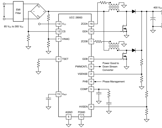
Typical Application Diagram
