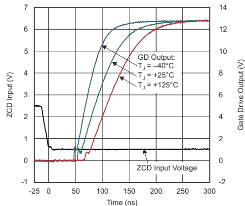
Figure 6-15. Gate Drive Rising and Delay From ZCD Input vs Time
