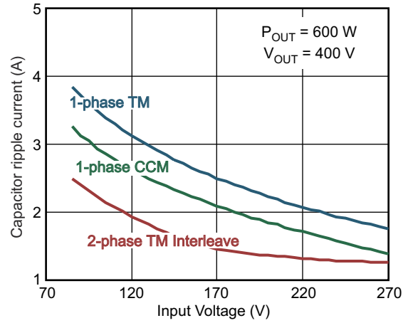
Input Ripple Current Reduction with Interleaving
