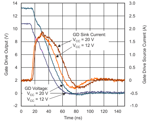
Figure 6-14. Gate Drive Falling vs Time
