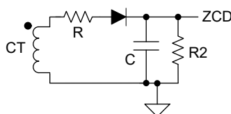
Figure 7-2. More Accurate Time Delay Circuit
