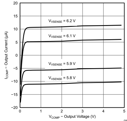
Figure 6-8. Error Amplifier Output Current vs Output Voltage
