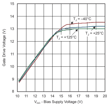
Figure 6-17. Gate Drive Output High vs VCC
