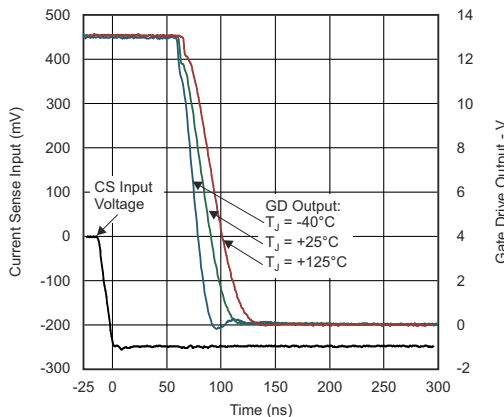
Figure 6-16. Gate Drive Falling and Delay From CS Input vs Time
