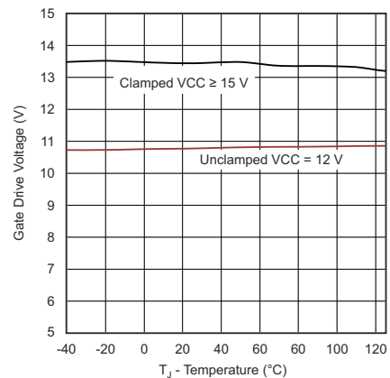
Figure 6-18. Gate Drive High Voltage vs Temperature
