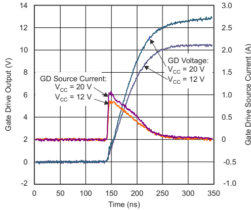
Figure 6-13. Gate Drive Rising vs Time
