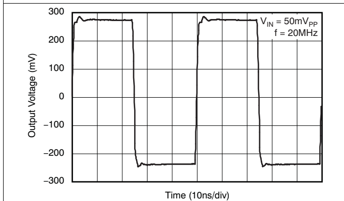
Figure 25. Small-Signal Pulse Response
