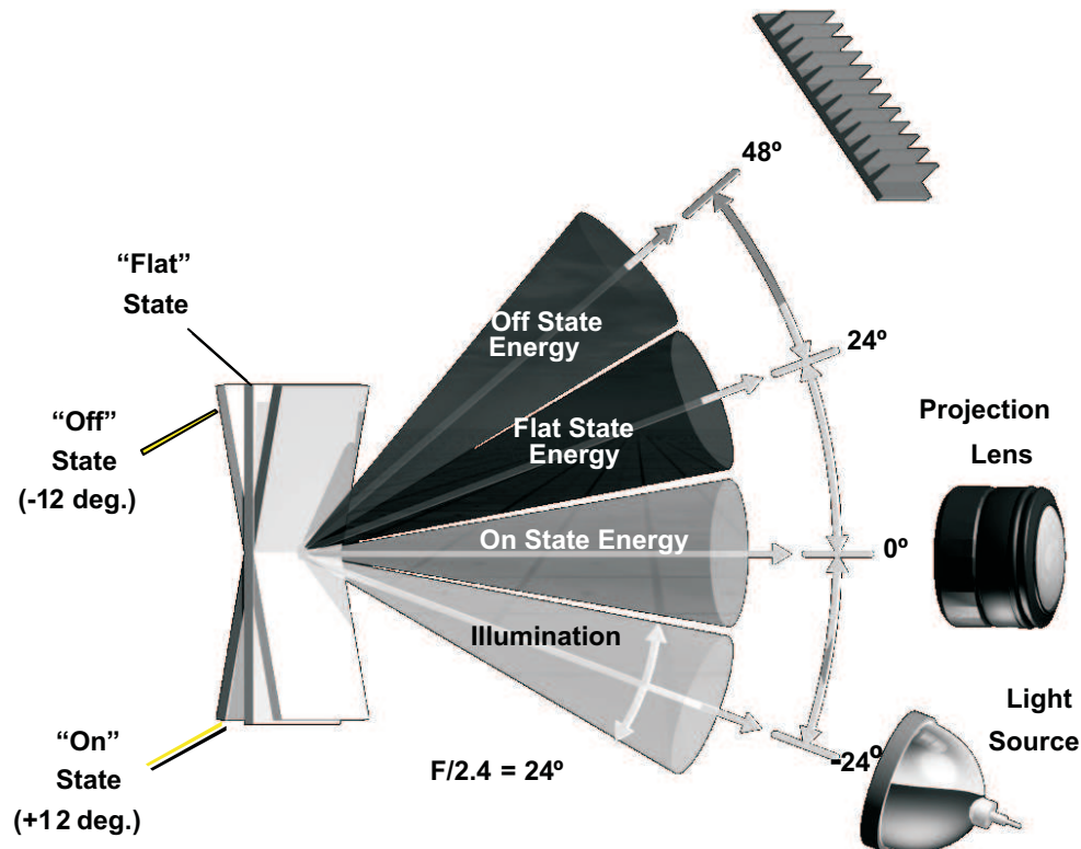
Figure 1. Simplified Optical Function of a 12-Degree-Mirror-Tilt Device
