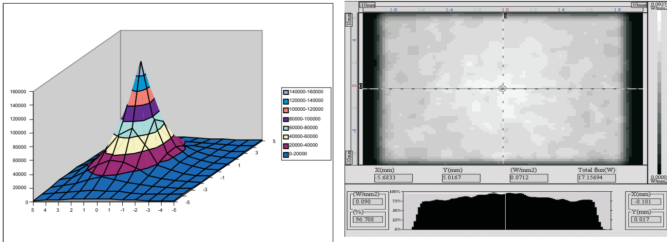
Figure 7. Spatial Irradiance Distribution of a Small-Arc Lamp at Focus of Elliptical Reflector Before Integration (left, at rod input) and After Integration (right, at rod output)
