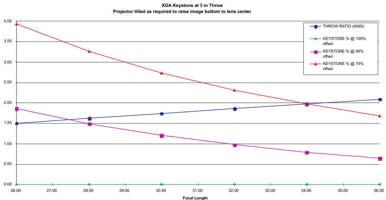
Figure 12. Keystone Distortion for 0.9 XGA by Throw Ratio and Offset
