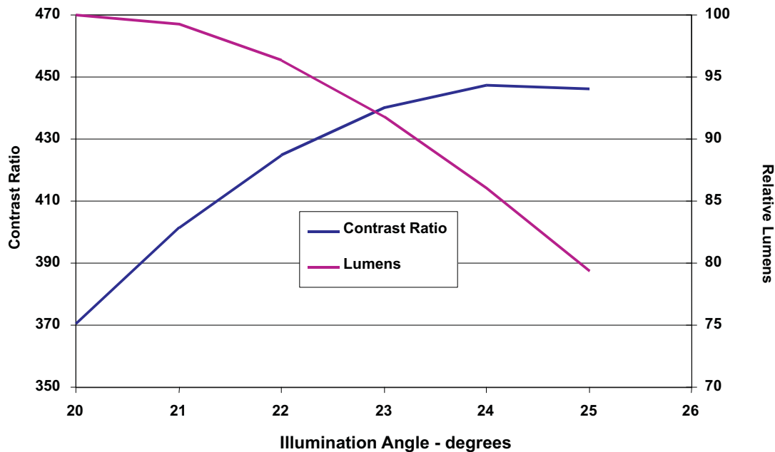
Figure 11. Contrast and Lumens as a Function of Illumination Angle for F/3 Telecentric System
