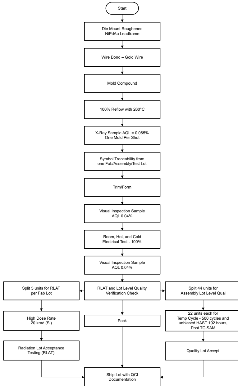
Figure 2-1. SN54SC2T74-SEP Space Enhanced Plastic Production Flow Chart
