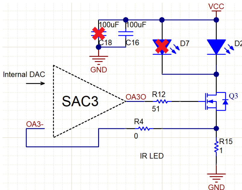
Figure 5. IR LED Driving Circuit With SAC
