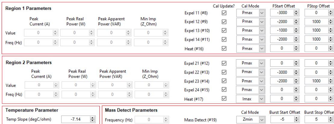
Figure 5-8. Calibration Settings and Parameters
