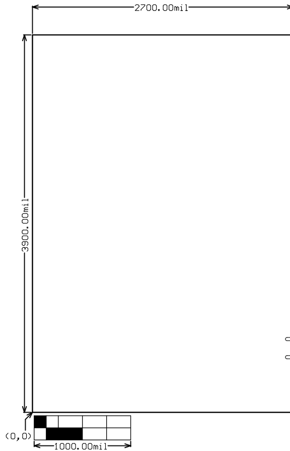
Figure 6-8. Board Dimensions
