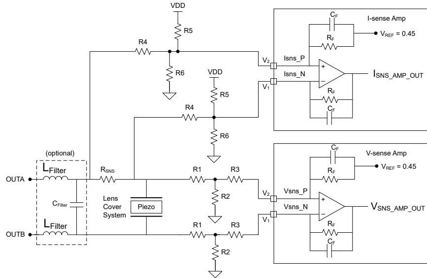
Figure 5-9. Voltage and Current Sense Amplifiers
