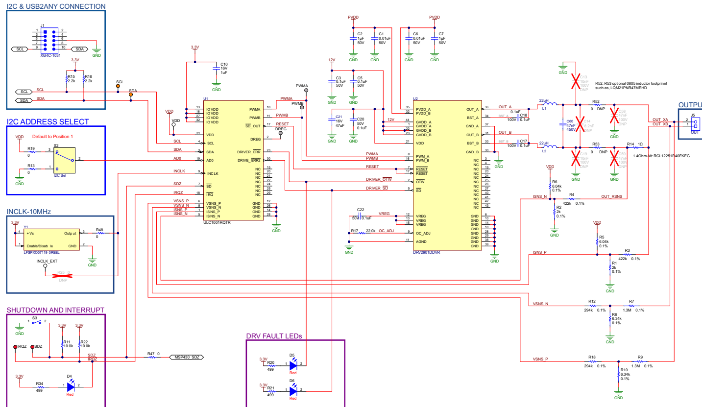
Figure 6-1. ULC1001-DRV290x EVM Schematic
