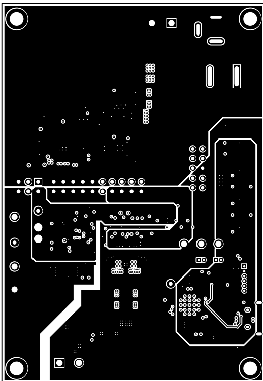
Figure 6-6. Signal Layer 2
