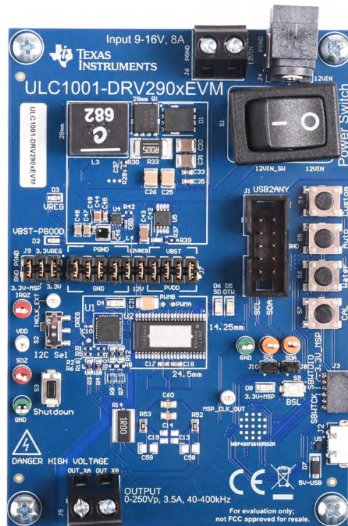
Figure 3-1. ULC1001-DRV290xEVM Top View
