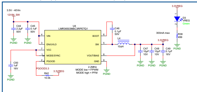
Figure 6-3. ULC1001-DRV290x EVM Power Supplies
