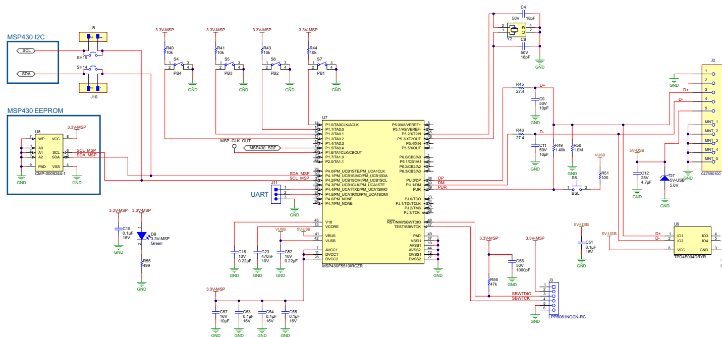
Figure 6-2. ULC1001-DRV290x EVM MSP430 Schematic
