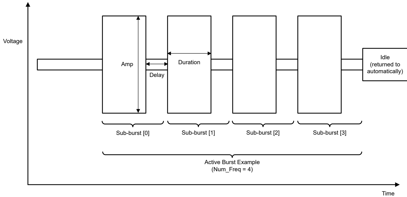
Figure 5-5. Active Burst Example
