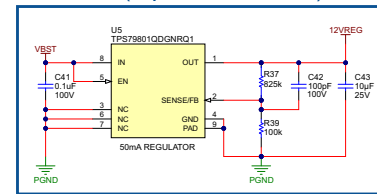
12V LDO (Input from Boost)
