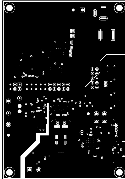
Figure 6-5. Signal Layer 1
