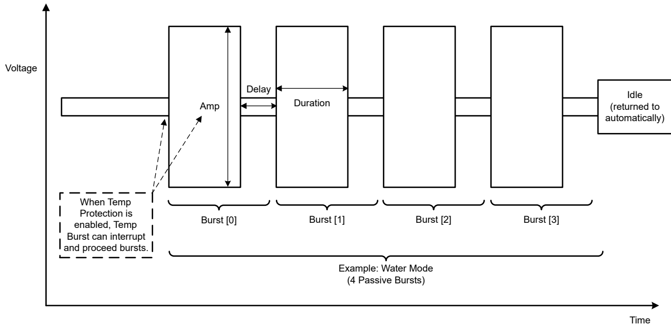
Figure 5-6. Passive Burst Example
