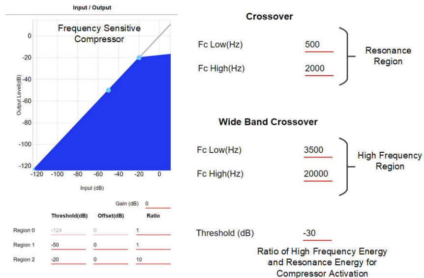
Figure 6-2. Rattle Noise Suppressor Controls
