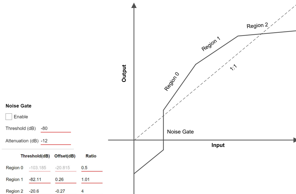
Figure 4-9. Controls for DRC Regions
