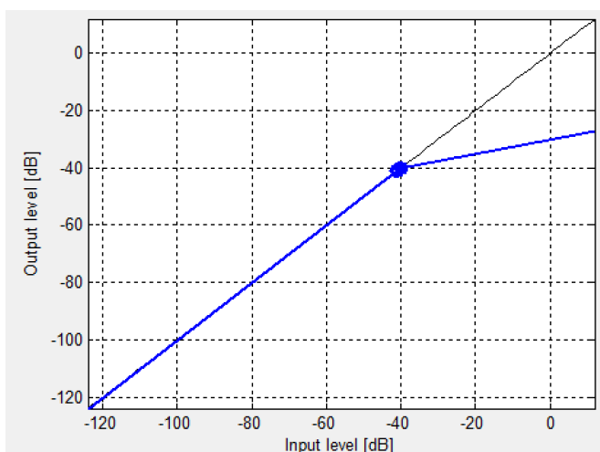
Figure 4-2. Compressor
