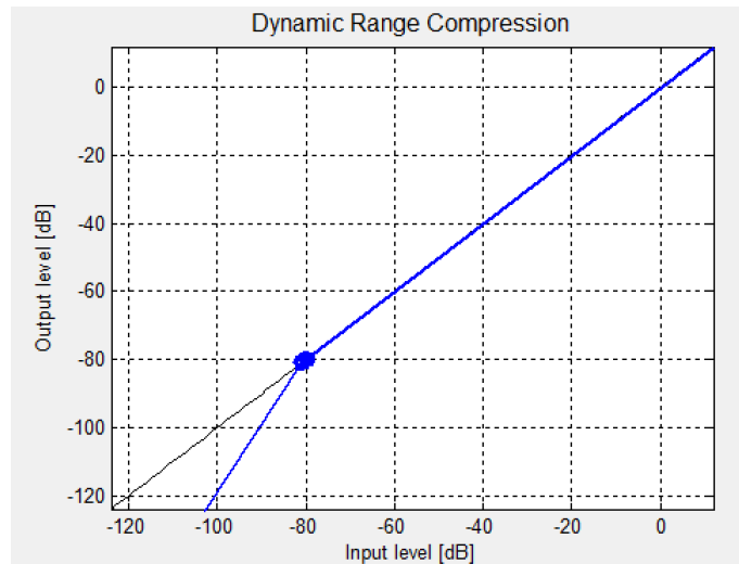
Figure 4-3. Expander
