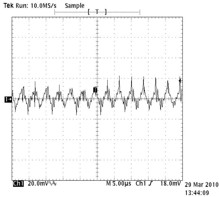
Figure 7. Output Ripple
