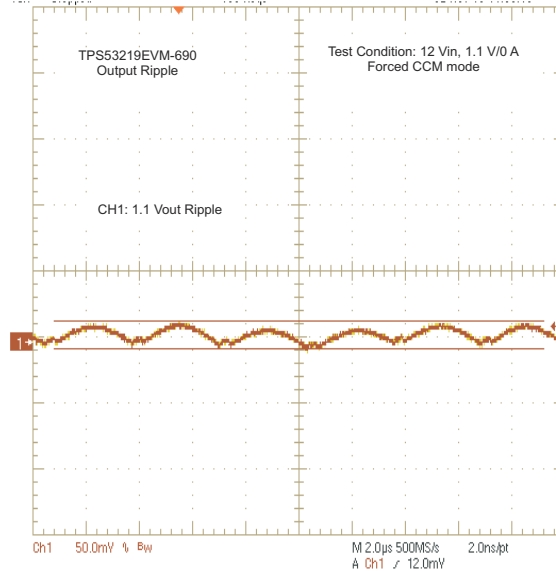
Figure 7-5. Output Ripple
