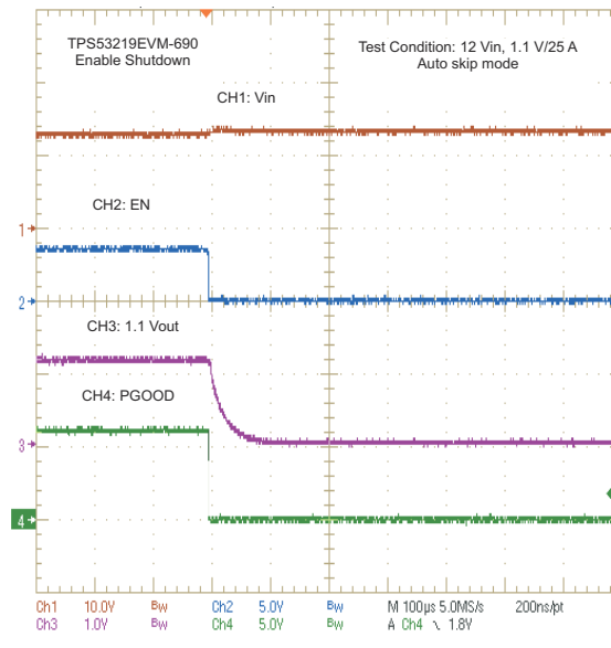
Figure 7-8. Enable Turn-Off
