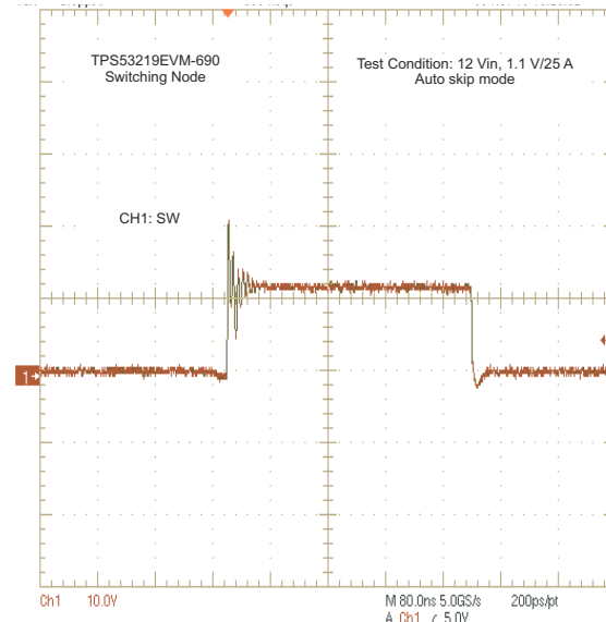
Figure 7-6. Switching Node
