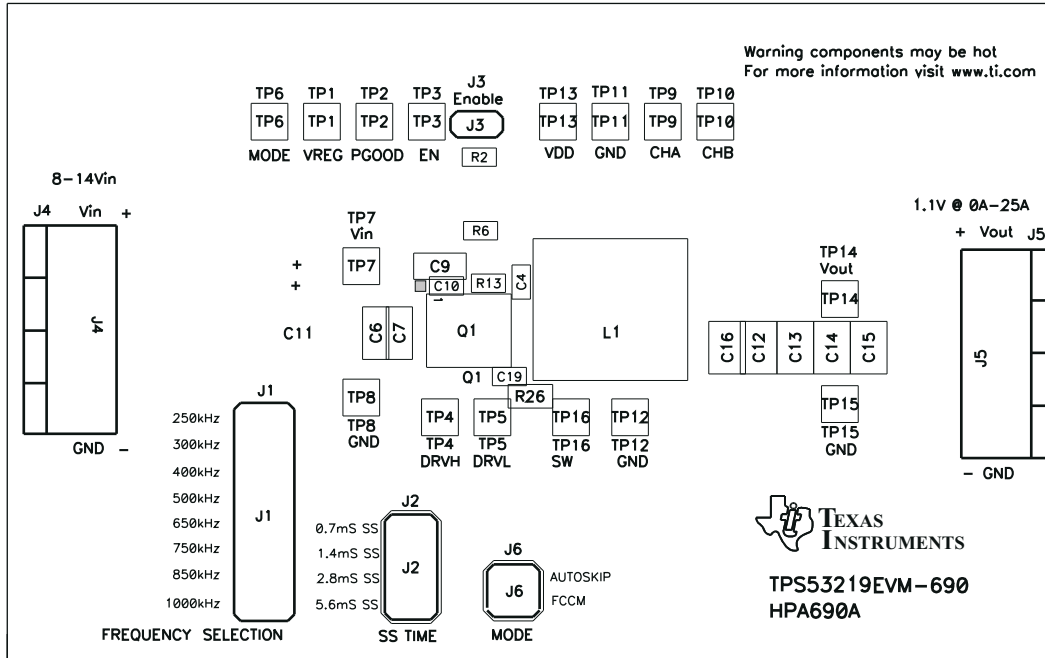
Figure 8-1. TPS53219EVM-690 Top Layer Assembly Drawing, Top View
