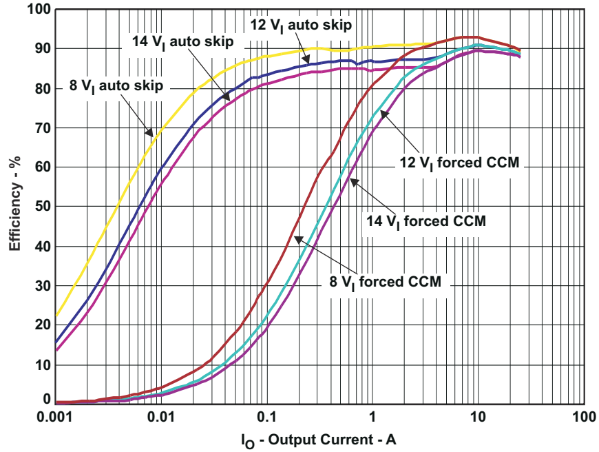
Figure 7-1. Efficiency
