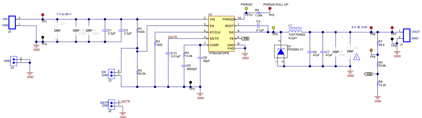
Figure 2. TPS54361EVM-555 Schematic
