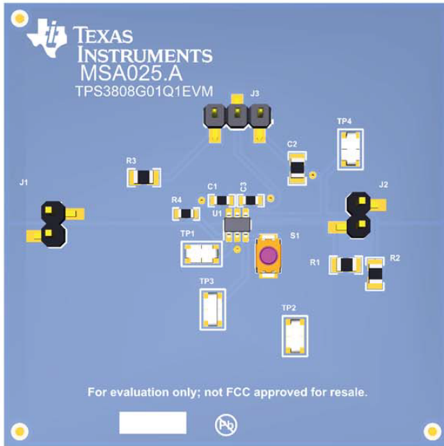
Figure 3. Component Placement—Top Assembly
