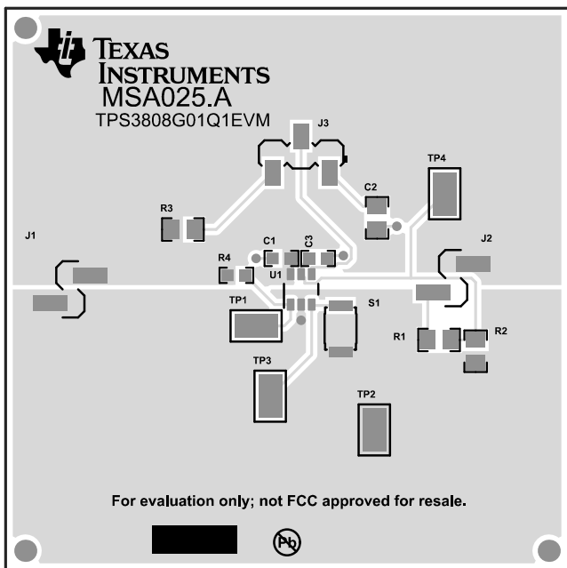
Figure 5. Layout—Top
