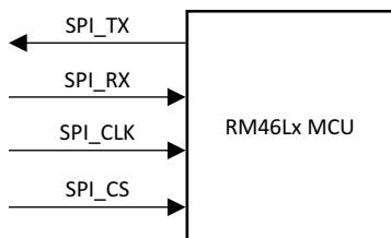
Figure 1. SPI Connections for RM46 Bootloader
