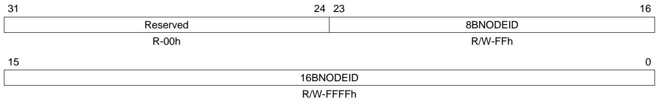
Figure 68. RapidIO DEVICEID1 Register (DEVICEID_REG1) - Address Offset 0080h
