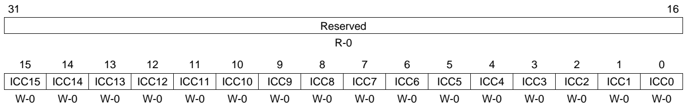
Figure 80. RX CPPI Interrupt Condition Clear Register (RX_CPPI_ICCR) - Address Offset 0248h
