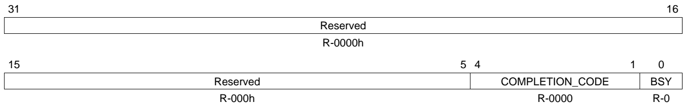
Figure 100. LSU n Control Register 6 (LSU n _REG6)
