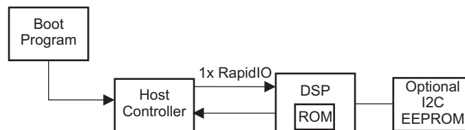
Figure 40. Bootload Operation
