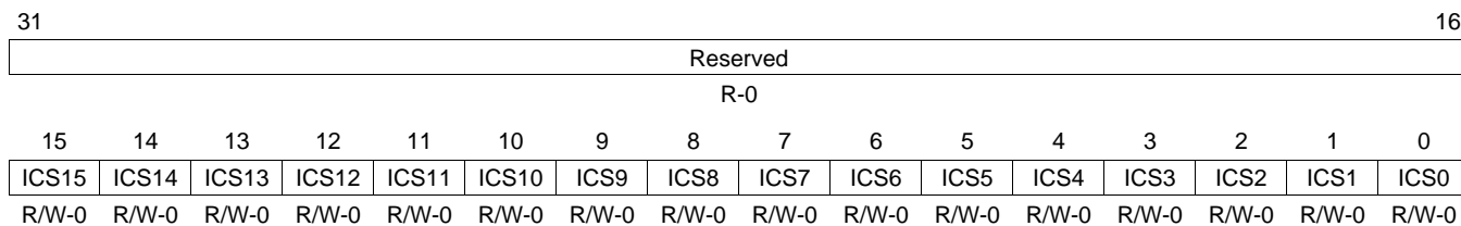
Figure 79. RX CPPI Interrupt Condition Status Register (RX_CPPI_ICSR) - Address Offset 0240h
