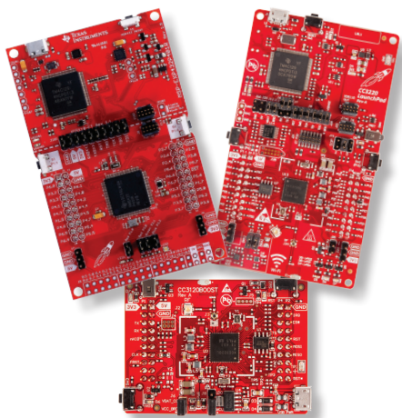
Figure 4. LaunchPad development kits offer complete development access to a SimpleLink MCU.
