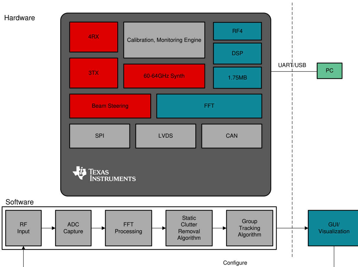
Figure 1. Hardware Block Diagram
