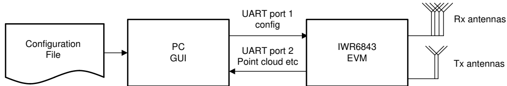
Figure 8. IWR6843 UART Communication
