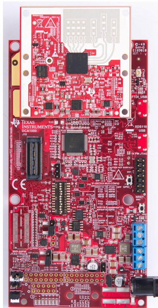
Figure 15. IWR6843ISK EVM
