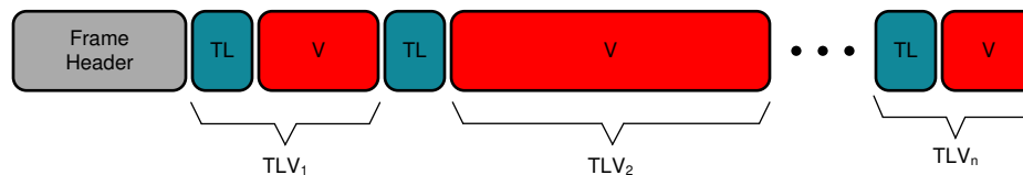
Figure 9. Output Frame Format
