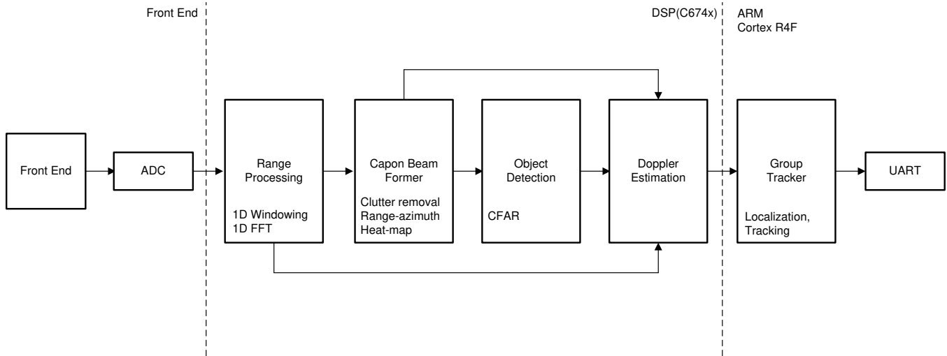
Figure 3. Automated Doors Application Block Diagram
