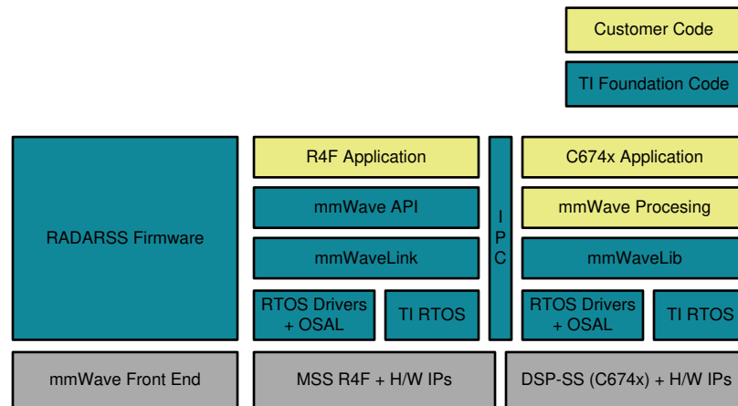
Figure 2. mmWave SDK Software Block Diagram
