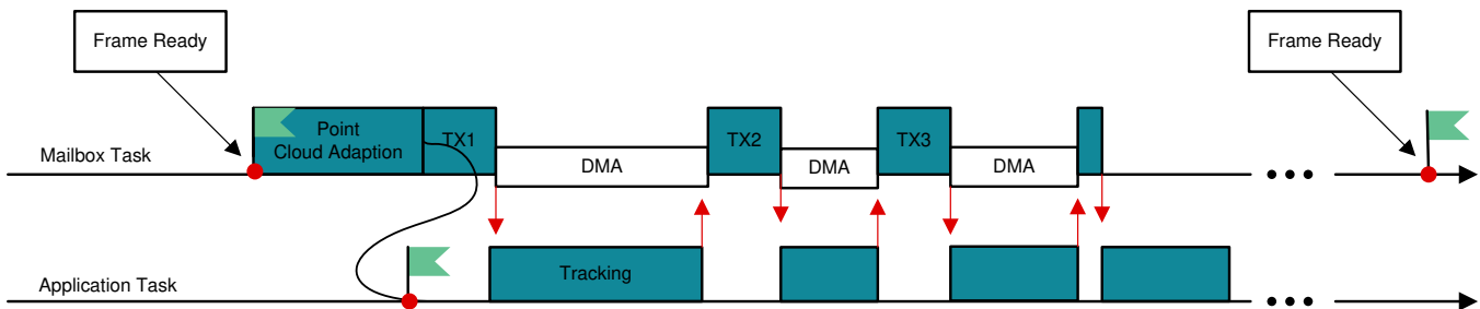
Figure 6. High-Level Processing Task Model
