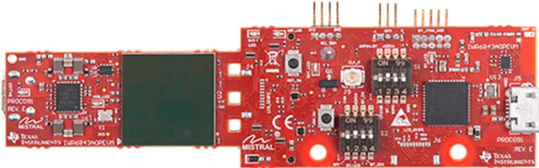
Figure 14. IWR6843AOP EVM
