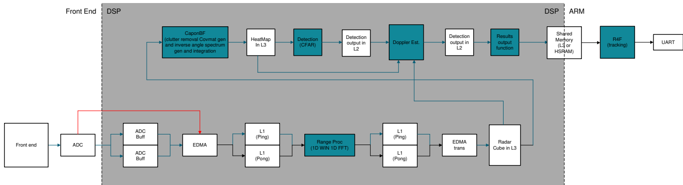
Figure 5. Processing Chain Flow: Detection-Tracking Visualization
