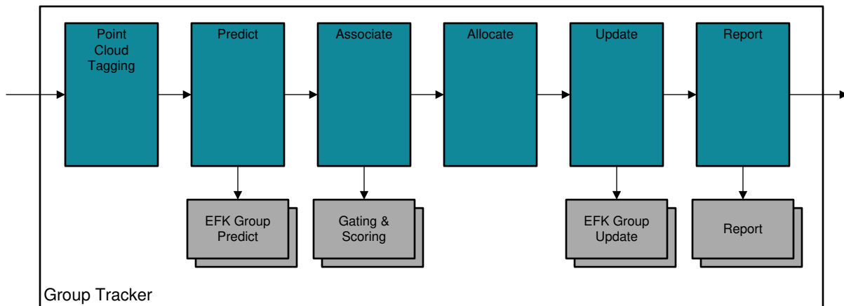
Figure 7. Group Tracking Algorithm
