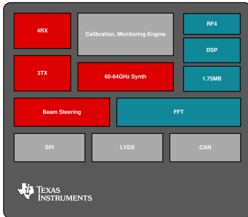
Figure 4. IWR6843 Block Diagram
